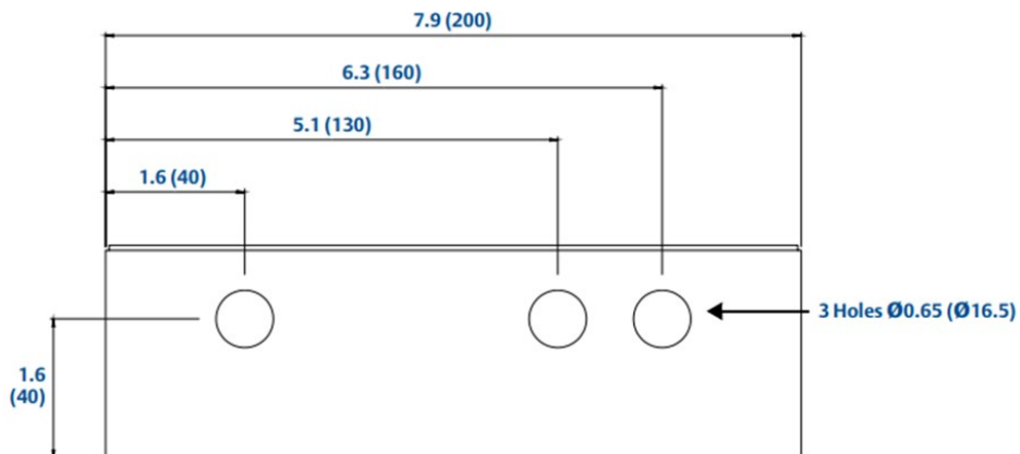
BOTTOM VIEW
